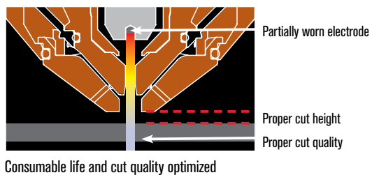
Proper cut height automatically maintained by the THC
