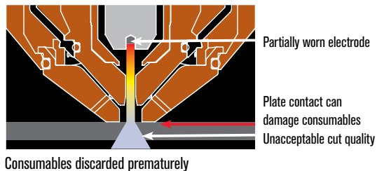
Improper cut height due to not adjusting arc voltage for electrode wear
